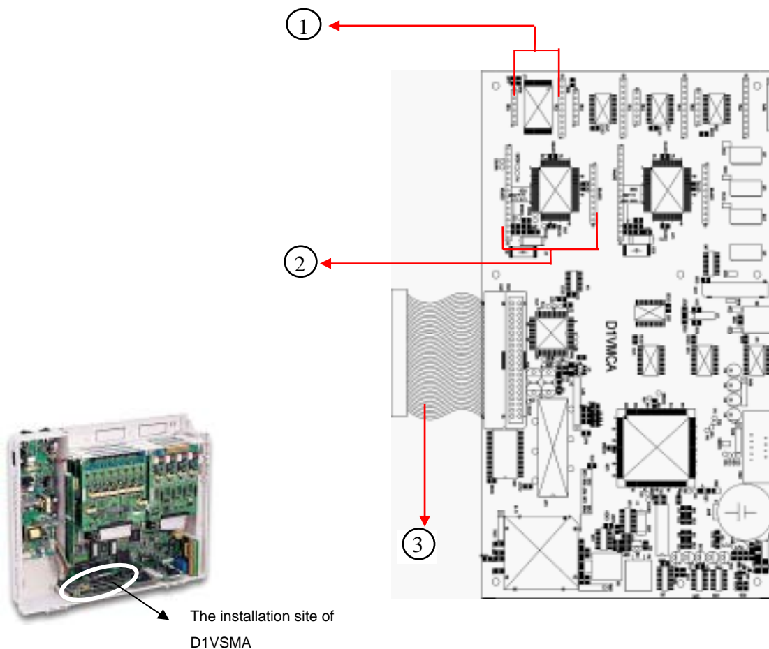
Figure 15. D1VMCA (Voice Mail Card)
