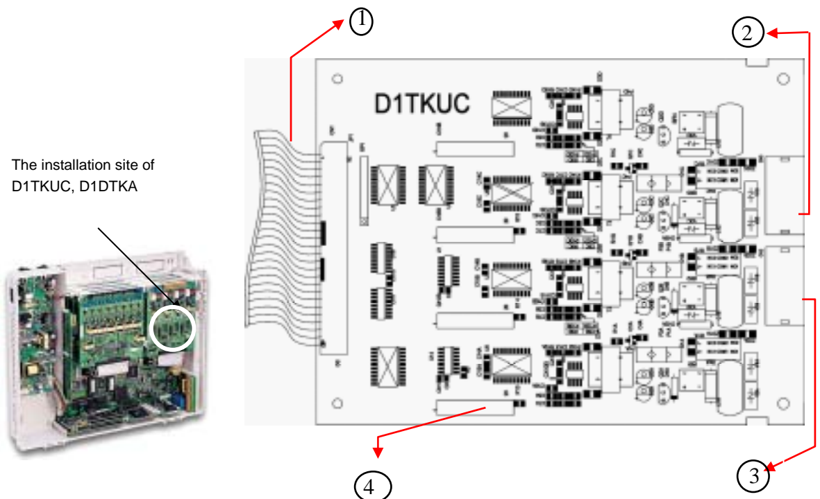
Figure 4. D1TKUC (TRUNK UNIT, 4 TRUNK PORTS)
