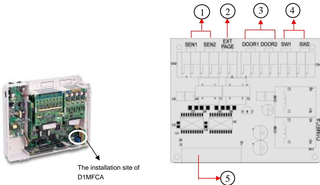
Figure 11. D1MFCA (Multi Function Card, 2 Sensor + 2 Relays + 2 Door Phones)
