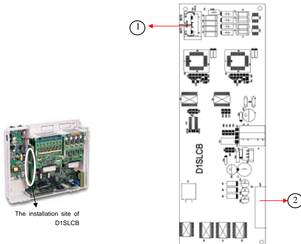
Figure 8. D1SLCB (Single Line Station Card, 4 SLT Station Ports)
