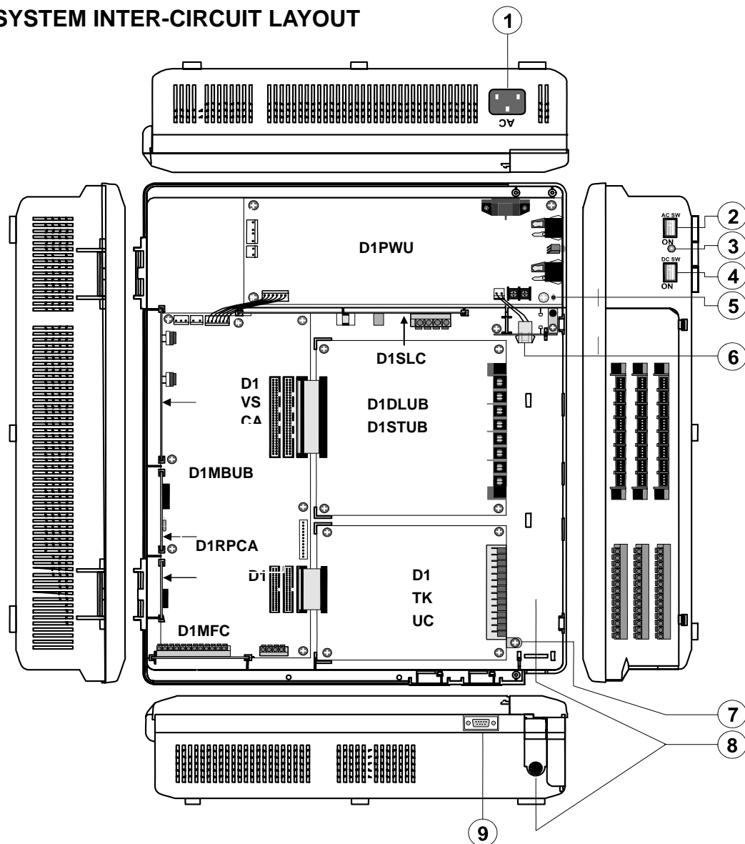
Figure 1. System Inter-Circuit Layout
