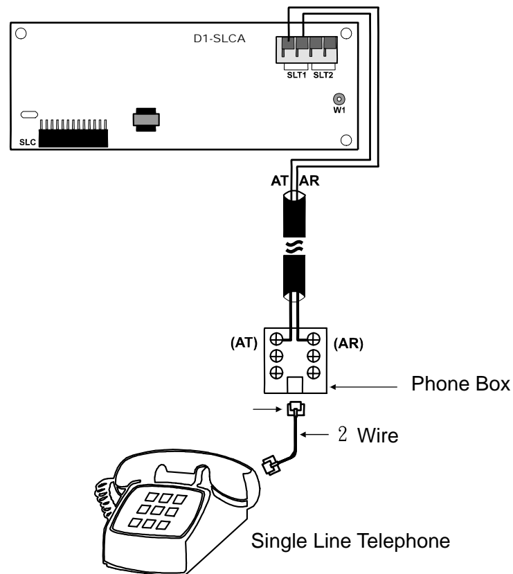
Figure 23. SLT Station Wiring on D1SLCB
