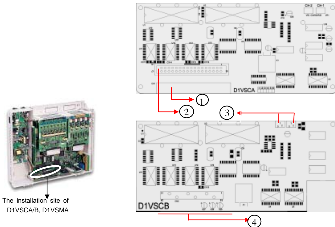
Figure 10. D1VSCA/B (VOICE SERVICE CARD, 2 VOICE CHANNEL)
