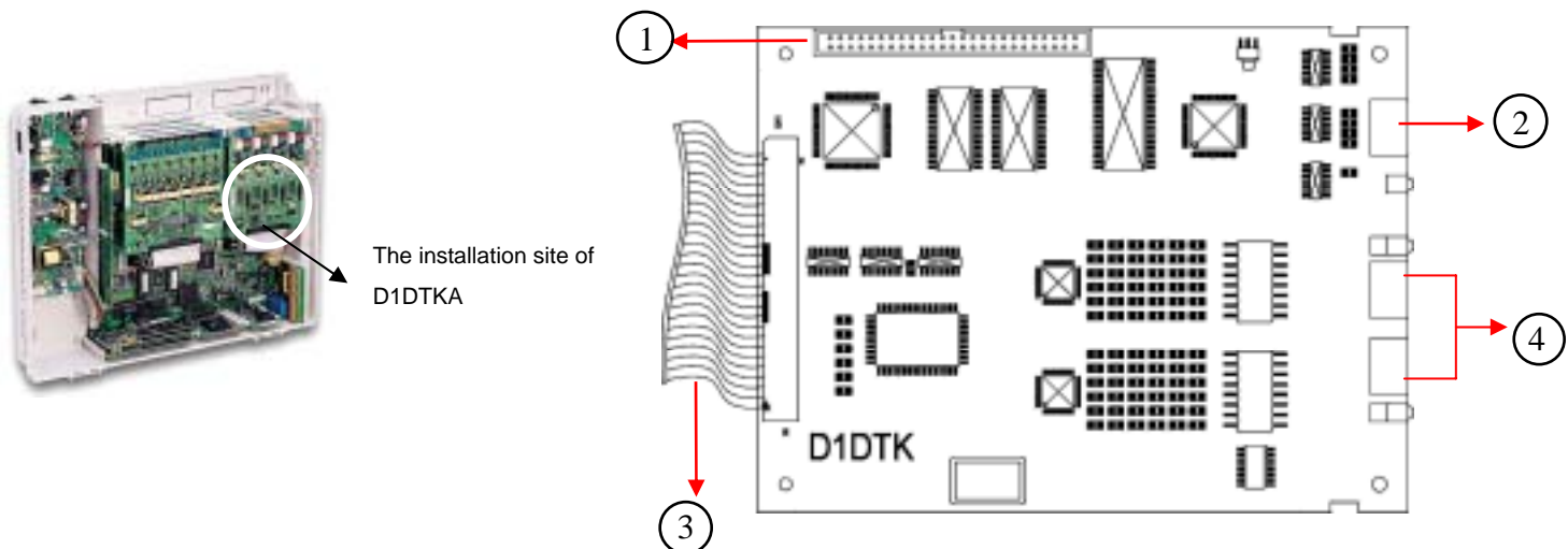
Figure 5. D1DTKA (ISDN TRUNK UNIT, 2 BRI PORTS)
