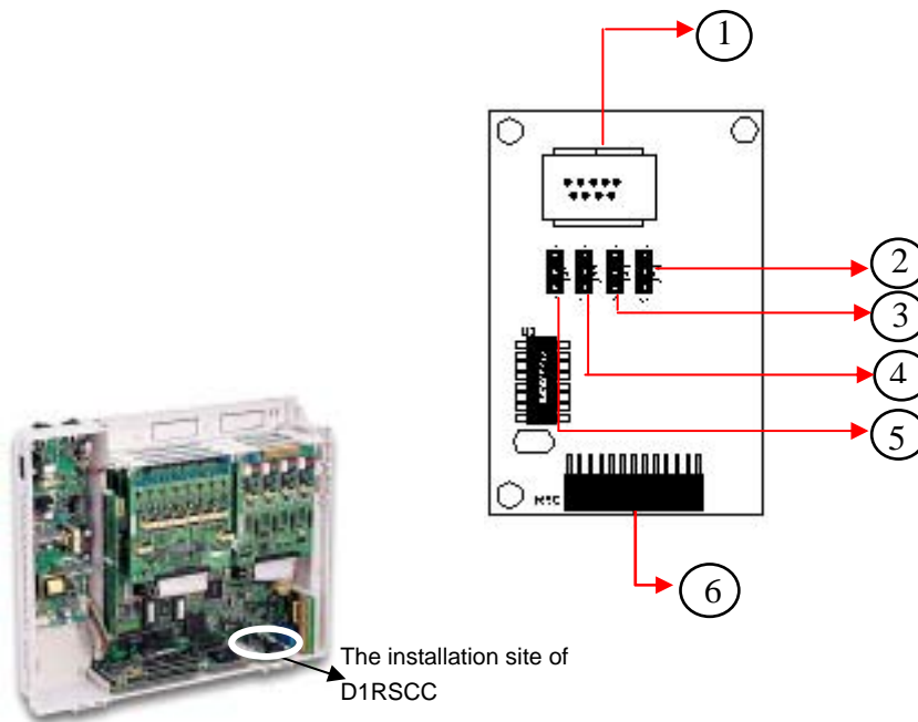
Figure 9. D1RSCC (RS232 Card, 2400bps Serial RS232 Port)
