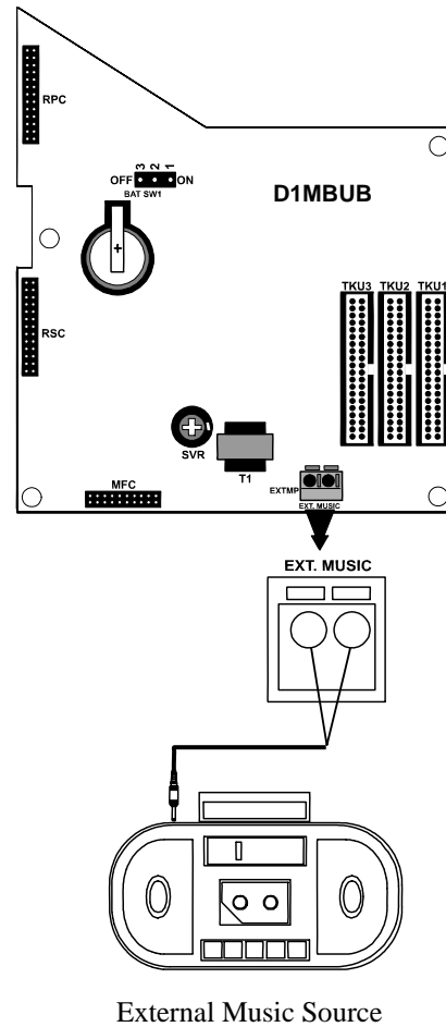
Figure 27. External Music Source Wiring on D1MBUB
