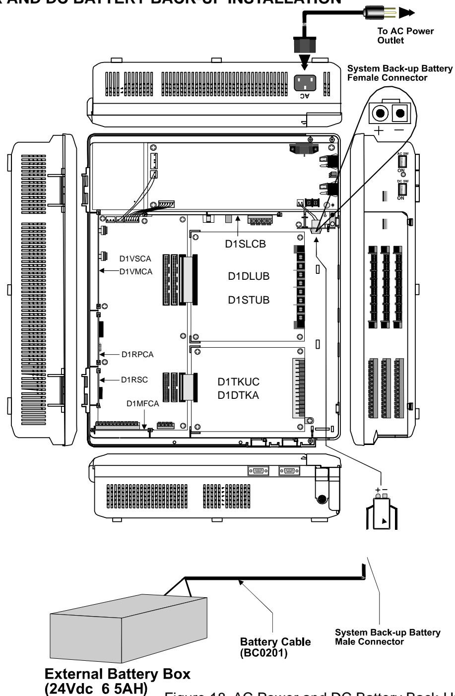
Figure 18. AC Power and DC Battery Back-Up Installation
