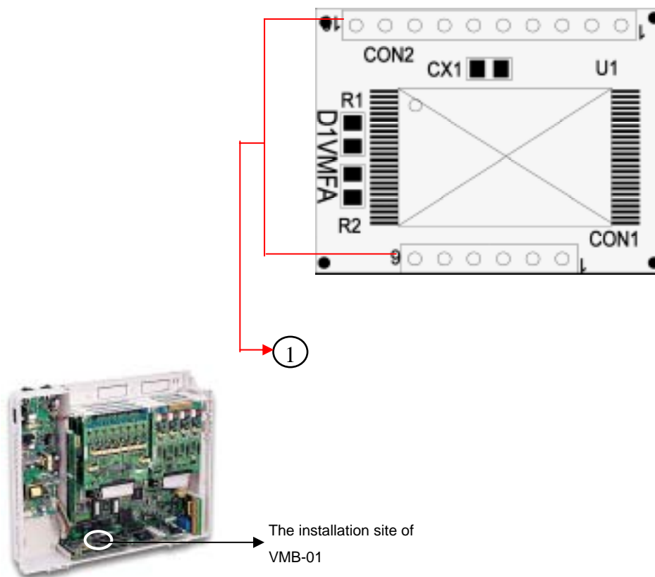
Figure 17. VMB-04 (Expansion Flash Memory)
