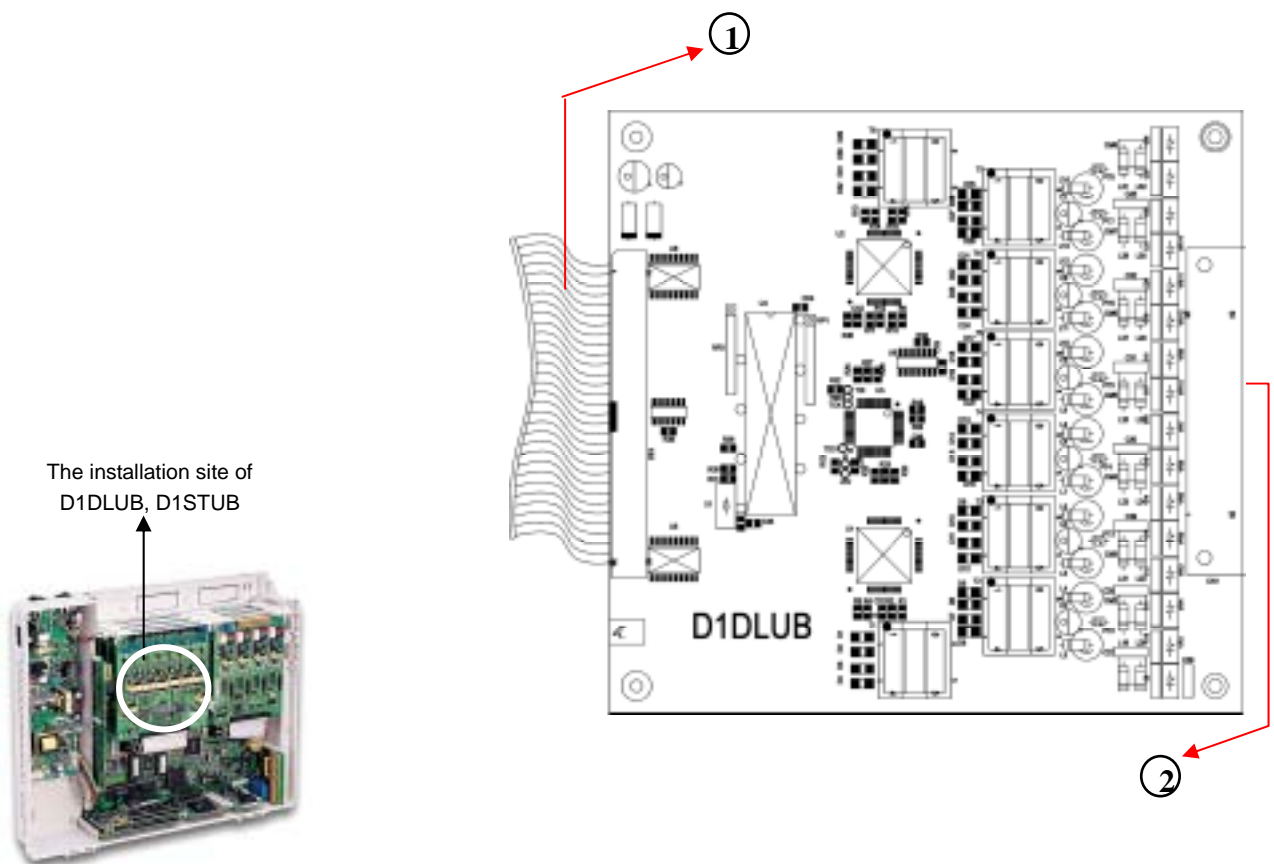
Figure 6. D1DLUB (Digital Key Station Unit, 8 Key Station ports)
