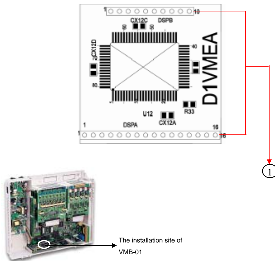
Figure 16. D1VMEA (Voice Mail Expansion Card)
